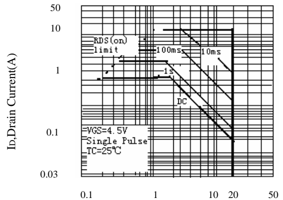
VDS, Drain-Source Voltage(V) Figure10.Maximum Safe Operating Area
